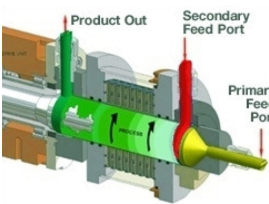
Spinning Tube-in-Tube Reactor
